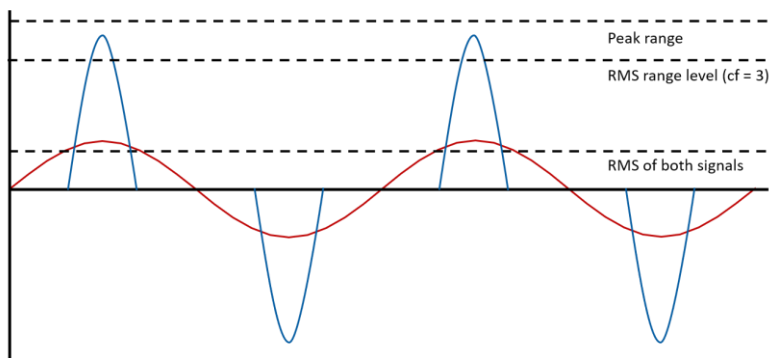
Figure 3: Comparison of two signals with same RMS value and different crest factors
